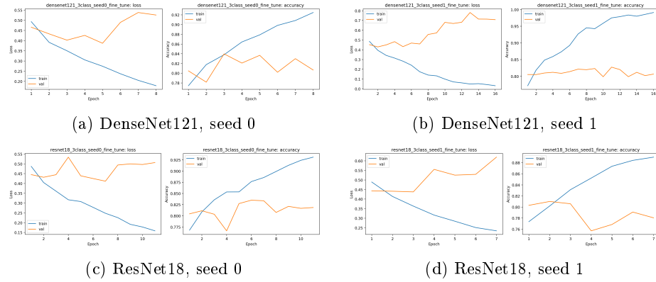
Fig. 9: Three-class fine-tuning curves (representative seeds) for both backbones.
