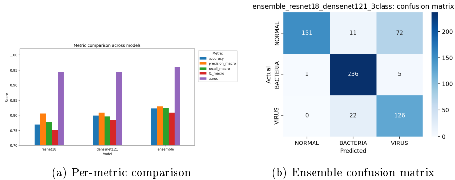
Fig. 5: Three-class results. (a) DenseNet121 and the ensemble dominate ResNet18 on every macro-averaged metric. (b) The dominant error is 72 NORMAL images predicted as VIRUS; BACTERIA is recognised almost perfectly.
