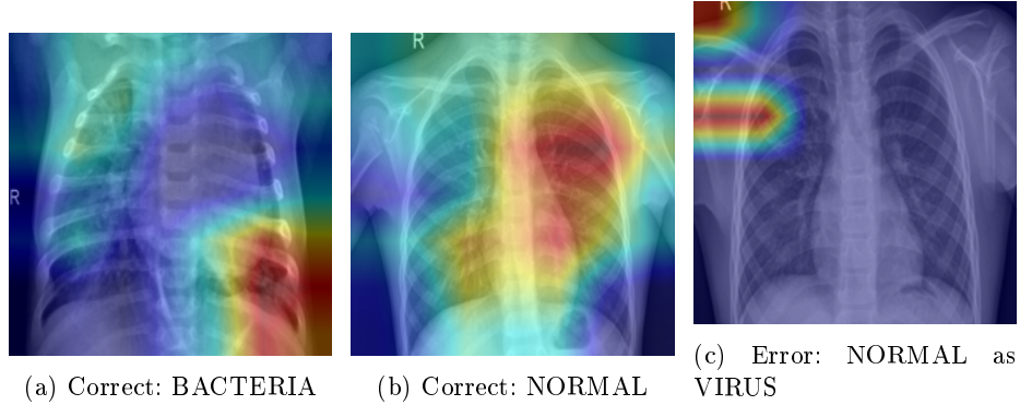
Fig. 8: Three-class Grad-CAM overlays (DenseNet121). Correct predictions (BACTERIA, NORMAL) focus on the relevant regions; the failure case shows a normal lung misread as viral pneumonia (diffuse activation), the dominant NORMAL→VIRUS error. The model produces no clean correctly-classified VIRUS example, consistent with viral pneumonia being the hardest class.
