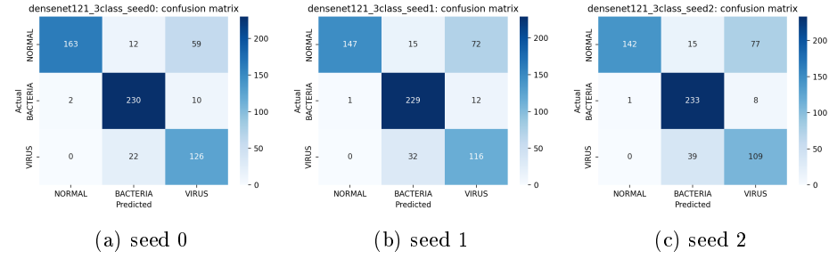
Fig. 10: Per-seed three-class confusion matrices for DenseNet121.
