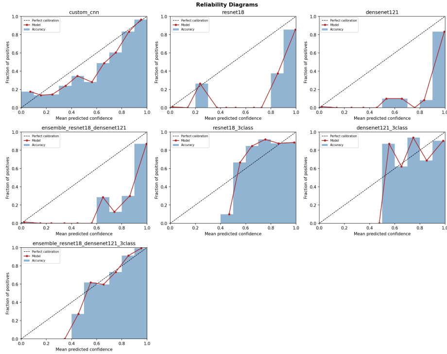
Fig. 6: Reliability diagrams. The dashed diagonal is perfect calibration; points above the diagonal indicate under-confidence and below it over-confidence. Transfer-learning models concentrate their predictions in the high-confidence bins.
